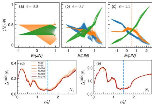
FIG. 10. Eigenstate expectation values for (N_1)_{\alpha,\alpha} (blue), (N_2)_{\alpha,\alpha} (orange), and (N_3)_{\alpha,\alpha} (green) as a function of energy, for \epsilon/J = 0.0 (a), \epsilon/J = 0.7 (b), and \epsilon/J = 1.5 (c); N = 270 . Average relative deviation of the eigenstate expectation values of N_1 with respect to the microcanonical average (d) and the normalized extremal fluctuations of the eigenstate expectation values of \hat{N}_1 (e) both as a function of the integrability breaking term \epsilon . In (d) and (e), the eigenstates lie in the energy range [E/(JN) - \Delta E/(JN), E/(JN) + \Delta E/(JN)] with E/(JN) = 0.5 and \Delta E/(JN) = 0.1 .
