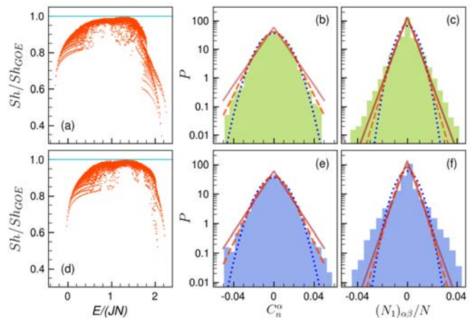
FIG. 14. Shannon entropy (a,d), distribution of the components of an eigenstate in the chaotic region (b,e), and distribution of the off-diagonal elements of the number operator of well 1 (c,f) for the bare Bose-Hubbard model (a)-(c) and the extended Bose-Hubbard model (d)-(f) in the positive parity sector; N = 180 . The parameters are the same as in Fig. 13. In (a,d): Solid line indicates the result for random matrix theory. In (b,c,e,f): Solid line represents the Laplace; dashed line, the Logistic; and dotted line, the Gaussian distribution. The best fit in (b) and (e) is the Logistic distribution. In (b), E/(JN) = 1.16 and in (e), E/(JN) = 1.33 .
