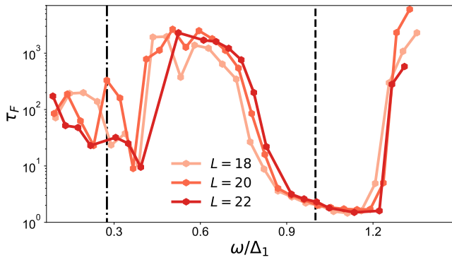
Figure 4. Half-time decay of the fidelity, \tau_F , as a function of the rescaled frequency \omega/\Delta_1 . The two vertical lines indicate the gaps \Delta_2 (dashed-dot) and \Delta_1 (dashed) for L = 22 . As in Fig. 1: initial state |\psi(0)\rangle = |11 \dots 11011 \dots 11\rangle , \alpha = 0.67 , J_x = 0.69 , h_x = 0.23 , h_y = 0.21 , and h_z = 0.19 .
